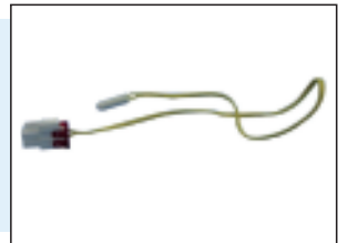
KOD NO.: 01 83 35 TERMOSTOP SF76E 76C 10 AMP 250 V 40 cm. (B2-031)
